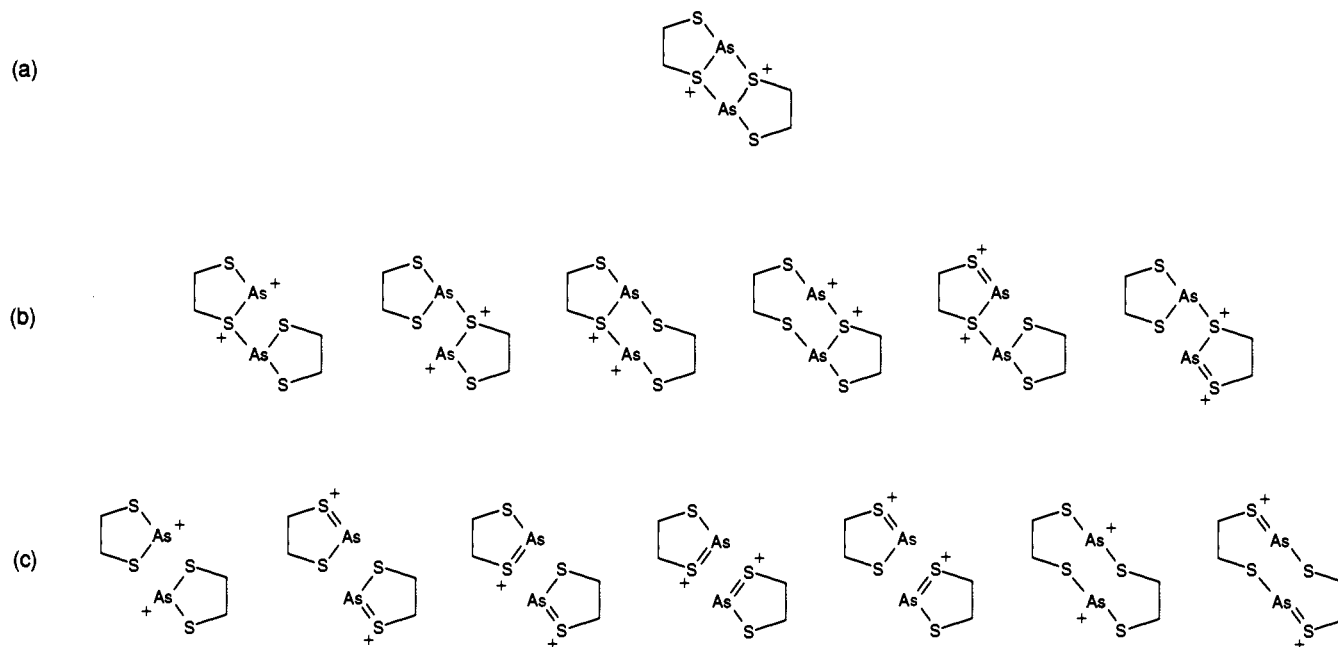
Figure 6. Principal resonance structures for [\text{SCH}_2\text{CH}_2\text{SAs}]_2^{2+} (5b).
