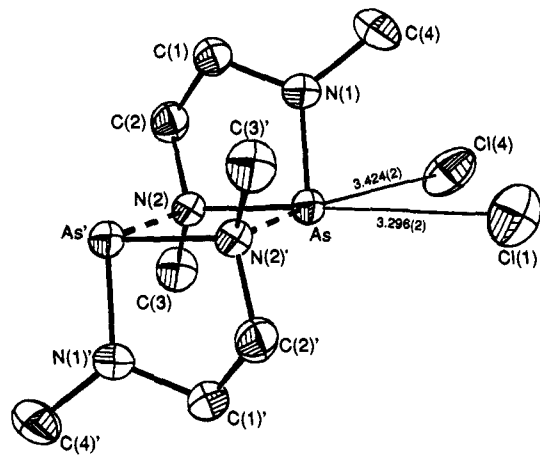
Figure 1. Crystallographic view of the cationic unit of [\overline{N(Me)CH_2CH_2N(Me)As}]_2 ( 5a ) [GaCl_4]_2 , showing anion-cation contacts.
