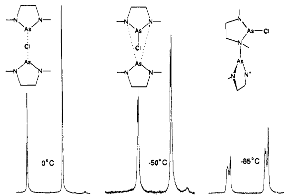
Figure 5. 1 H NMR spectra at 0, -50, and -85 °C for [N(Me)-CH 2 CH 2 N(Me)AsN(Me)As(Cl)N(Me)CH 2 CH 2 ] + ( 6a ) [GaCl 4 ] - , with topological models for the cation to rationalize each spectrum.
