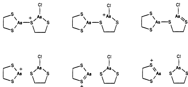
Figure 7. Principal resonance structures for [\text{SCH}_2\text{CH}_2\text{SAsSAs}(\text{Cl})-\text{SCH}_2\text{CH}_2]^+ (6b).
