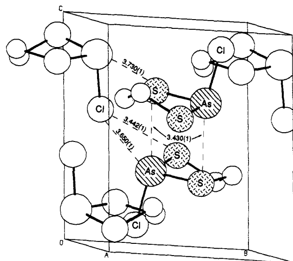
Figure 4. Crystallographic view of the unit cell of \overline{SCH_2CH_2SAAsCl} ( 4b ).
