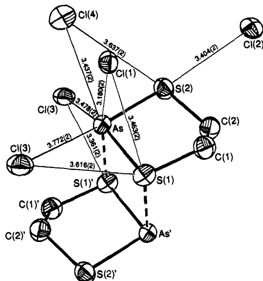
Figure 2. Crystallographic view of the cationic unit of [\overline{SCH_2CH_2SAs}]_2 ( 5b ) [GaCl_4]_2 , showing anion-cation contacts.
