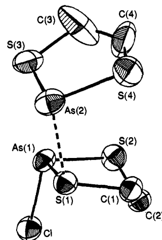
Figure 3. Crystallographic view of the cationic unit of [\overline{SCH_2CH_2S-AsSAs(Cl)SCH_2CH_2}] ( 6b ) [GaCl_4] .
